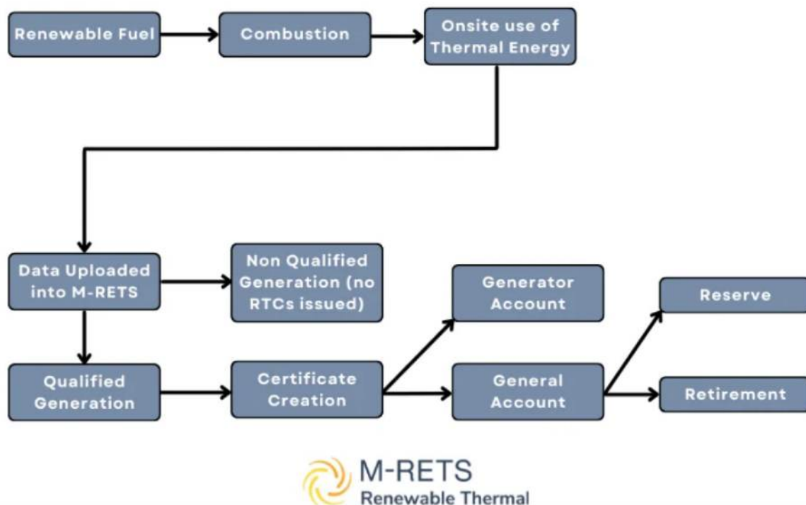
Figure 4: RTC Process for Combined Heat & Power Using Renewable Thermal Fuels
